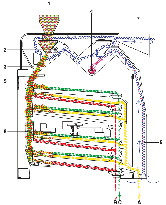
Function Diagram VC2222A
