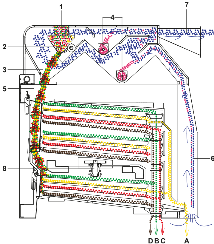
Function Diagram VC333A
