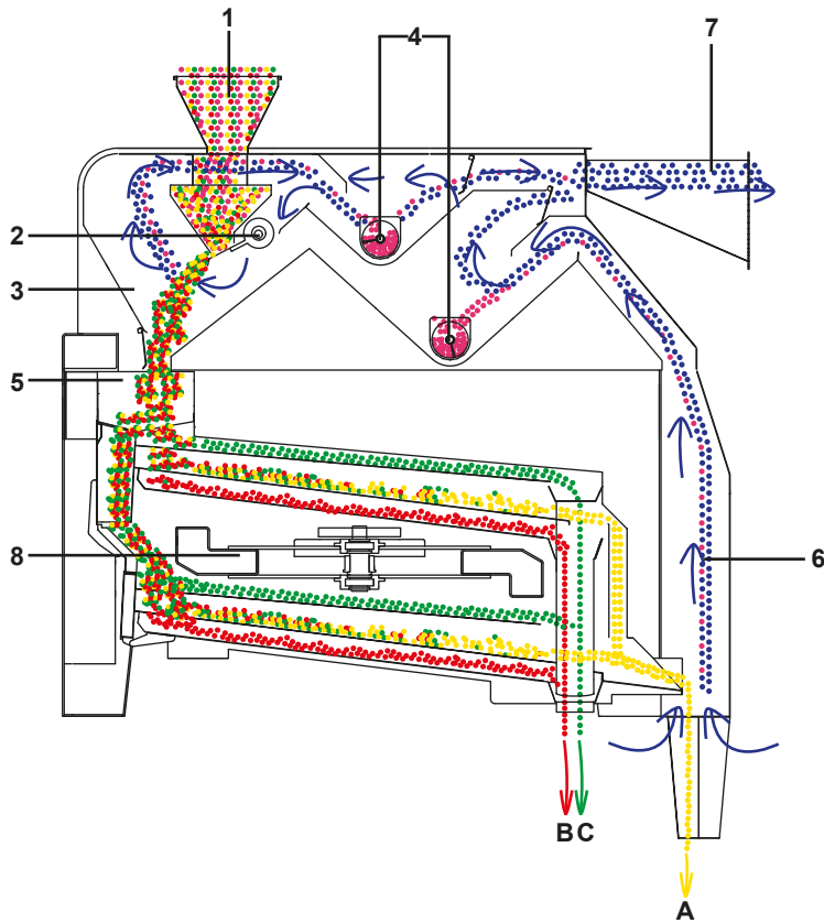
Function Diagram VC22A
